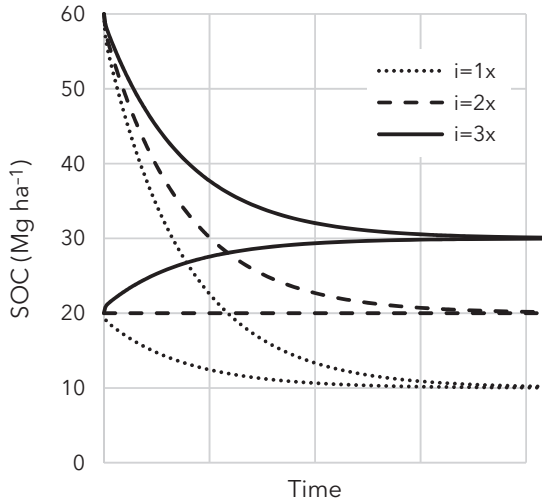
Figure 2 Soil organic carbon (SOC) dynamics in two hypothetical soils with different land use and management history, both receiving carbon inputs, i , at three different rates, 1x, 2x, and 3x (highest rate). In this example, we used a two-pool SOC model (ICBM; Andrén and Kätterer, 1997), but any other commonly used carbon model would produce similar curves. The soil with high initial SOC loses much more carbon over time than the soil starting with low initial SOC, but absolute differences in SOC between input rates are identical at any point in time, irrespective of initial conditions. Response ratio, i.e. the ratio of SOC stocks at different input rates, is dependent on both time and initial conditions. Only the low SOC soil at the highest input rate leads to net soil carbon sequestration, but carbon storage increases in both soils when input rates increase and both soils approach the same steady-state SOC stock when carbon inputs equal outputs.
